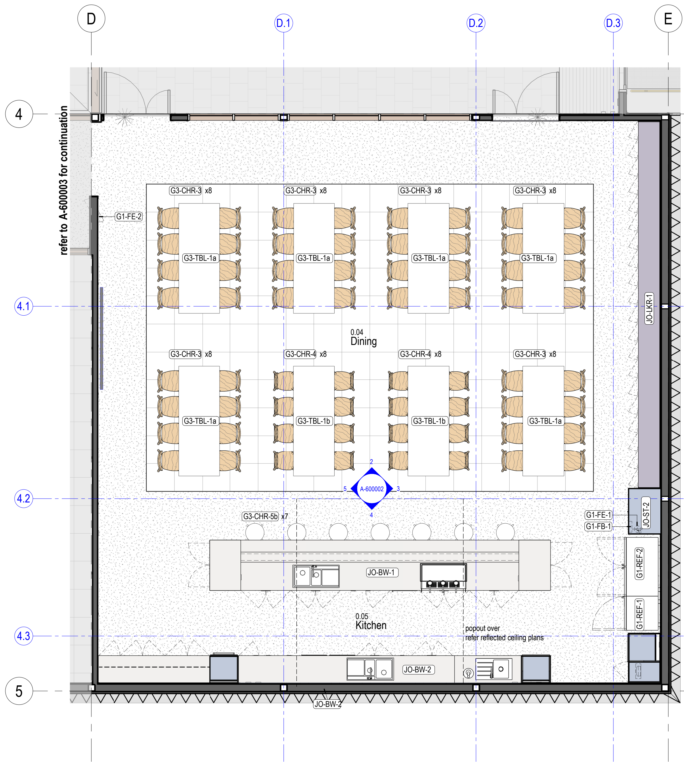
1 0.04-0.05 - Dining and Kitchen - Plan 1 : 50
