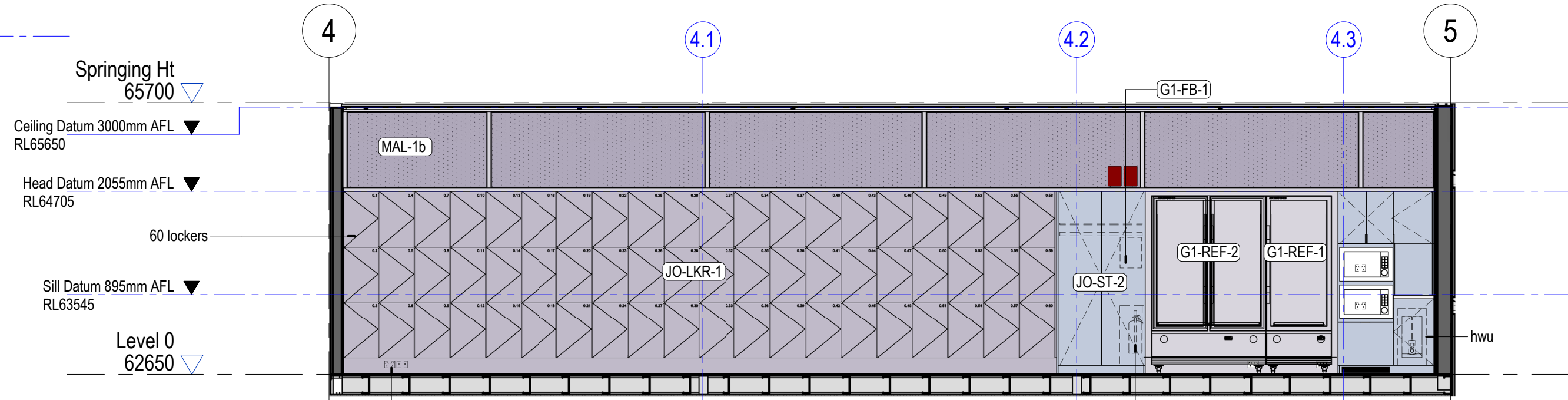
3 0.04 - Dining - East Elevation 1 : 50
