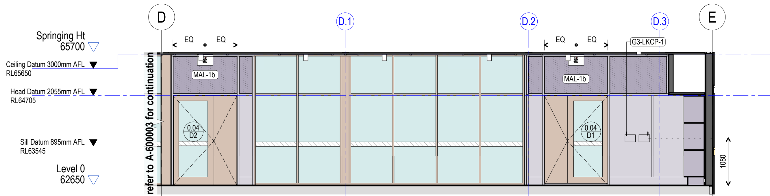
2 0.04 - Dining - North Elevation 1 : 50
