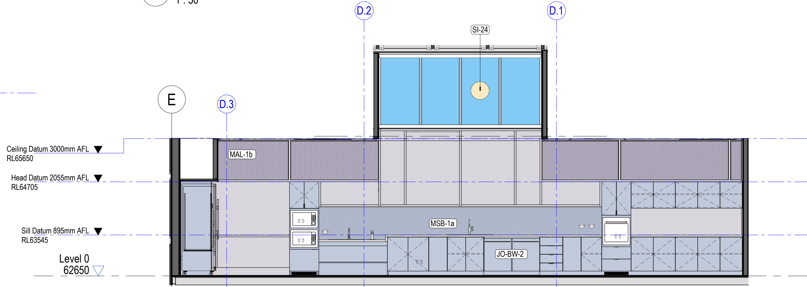
4 0.05 - Kitchen - South Elevation 1 : 50
