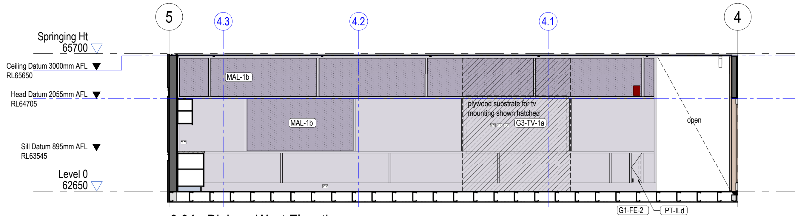
5 0.04 - Dining - West Elevation 1 : 50
